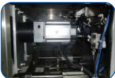
Servo Belt Film Drive
